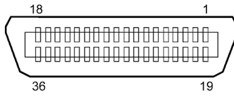
IEEE1284-B Connector
